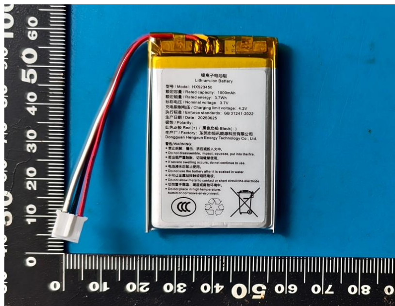
Fig. 2 – Back view of Battery
