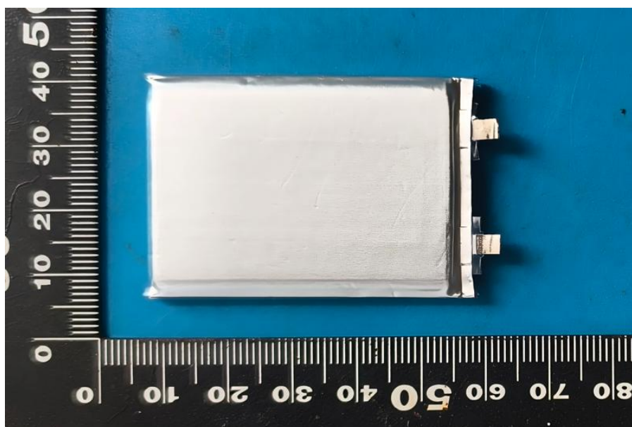
Fig. 4 – Back view of Cell 表4 – 电芯反面视图
