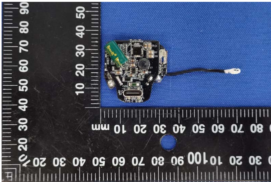
Figure 3 Front view of PCB
