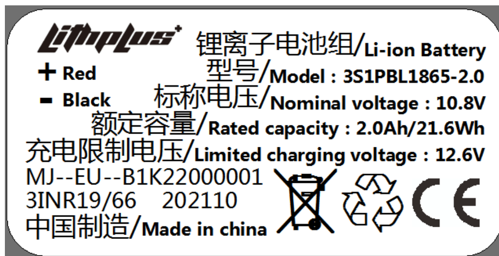
Figure 7 Battery label
